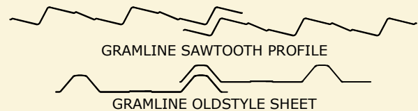
CORRECT OVERLAP DETAIL FOR THE INFILL SHEET PROFILES
